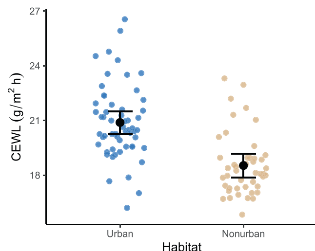
FIGURE 4 Urban Aegean Wall Lizards on the island of Naxos, Greece, exhibited significantly higher cutaneous evaporative water loss (CEWL) than their counterparts found in nonurban habitats. Smaller coloured points represent individual lizards, while larger black points represent estimated marginal means from our linear models with 95% confidence intervals.
