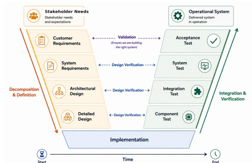
Figure 1. Systems Engineering V-Model. The model illustrates the relationship between system definition, engineering design, implementation, integration, verification, and validation.
